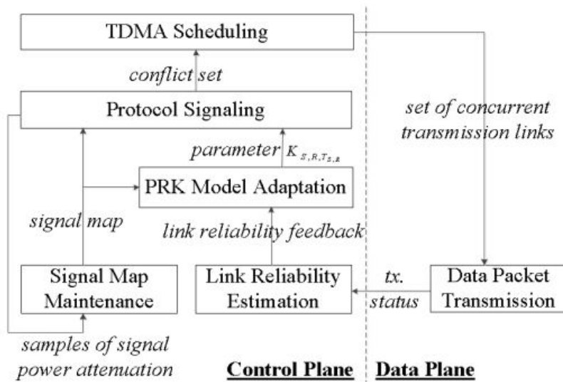
Fig. 2.4.2 PRKS Architecture Diagram (source [2]).
